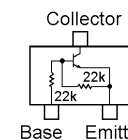
RT1N241M (N2) (Q1002, 1006, 1016, 1032, 1033, 1034, 1035, 1502, 1506, 1507, 1512, 1518)
